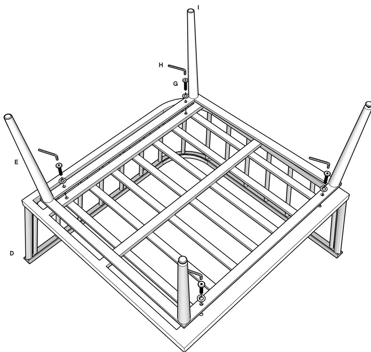
FRONT LEG
